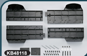
Chassis for decoration Fits 3 different width Used with 1/10 RC touring car
